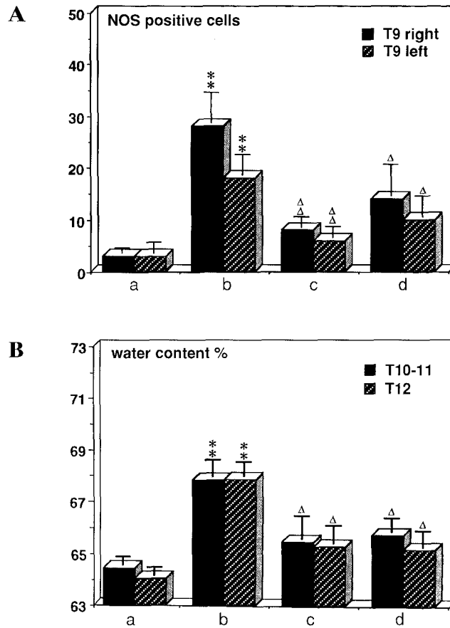
Fig. 2. A Semiquantitative analysis of NOS upregulation in the spinal cord following trauma and its modification by BDNF or IGF-1 treatment. B Water content following spinal cord injury and its modification with BDNF and IGF-1 treatment (** p < 0.01 , Student's unpaired t-test compared from control group; \Delta p < 0.01 , compared from spinal cord injury group). a control; b SCI; c BDNF + SCI; d IGF + SCI; SCI spinal cord injury
